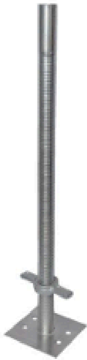
BASE JACK HOLLOW Plate 150×150×5 mm
