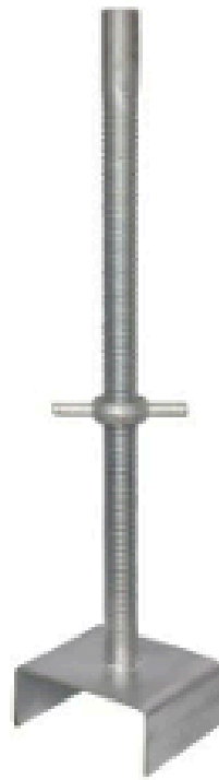
U HEAD JACK HOLLOW U-Head 150×170×190×5mm
